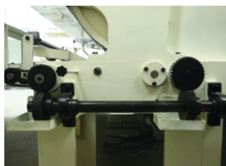
All Helical Gear Shaft Drive
