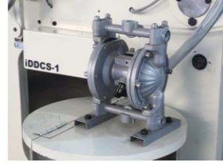
Intelligent Ink Circulating System with Ink Tank
